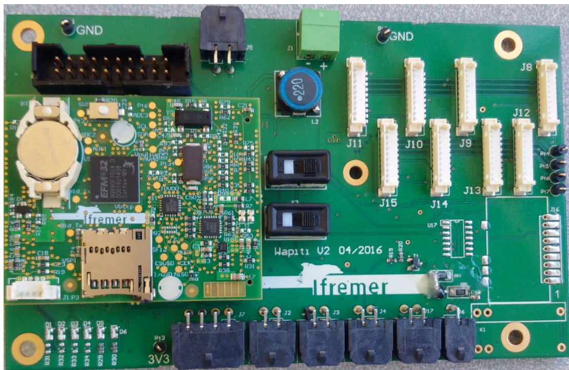
Picture 4. WAPITI and ALEES boards at the development stage in IFREMER
