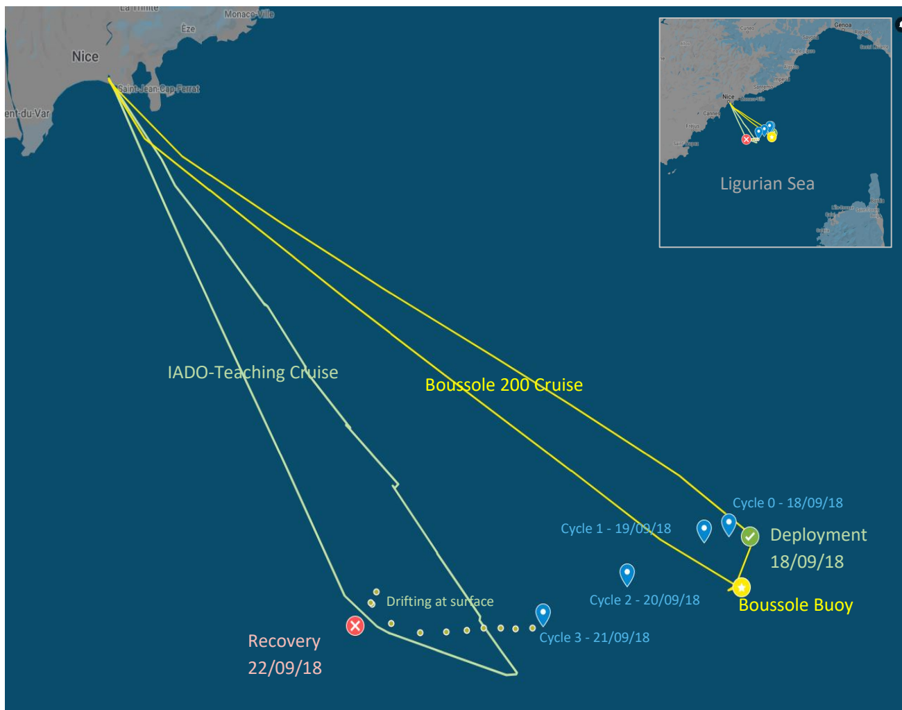
Figure 7. Deployment and recovery of the p\text{CO}_2 profiling float prototype in the Ligurian Sea during BOUSSOLE/MOOSE/IADO-Teaching cruise. Blue symbols are the float's location at the end of each corresponding cycle.
